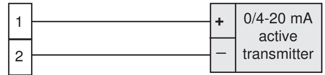
Fig. 10- 0/4-20 mA input wiring for active transmitter
